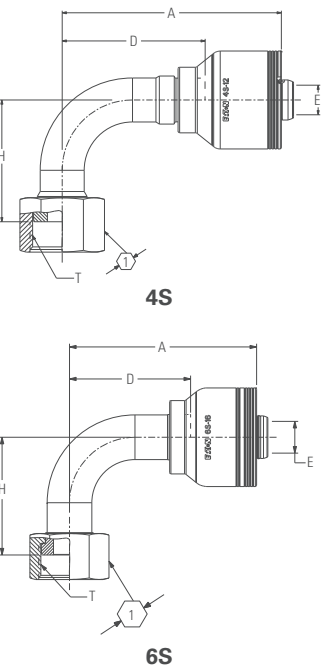
Female ORS Swivel (FRB) 90° Elbow
